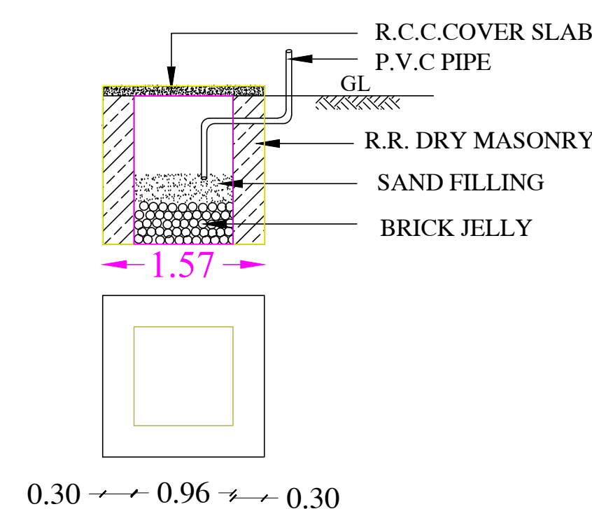
RAIN WATER HARVEST ARRANGEMENTS
