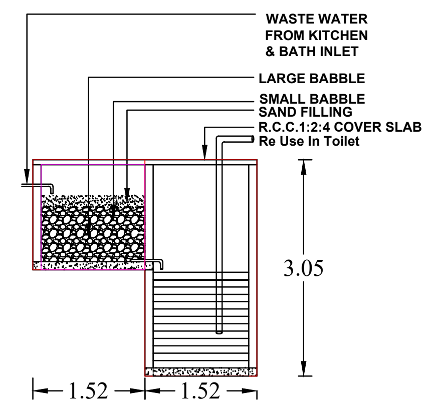
RECYCLING OF WASTE WATER FROM KITCHEN & BATHROOM
