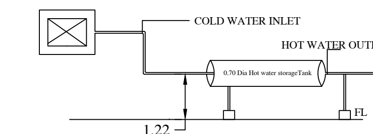
SOLAR WATER HEATING SYSTEM DETAILS
