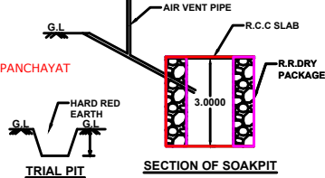
SECTION OF SOAKPIT
