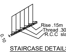
STAIRCASE DETAILS
