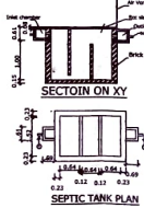
SEPTIC TANK PLAN
