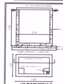
UG SUMP DETAILS
