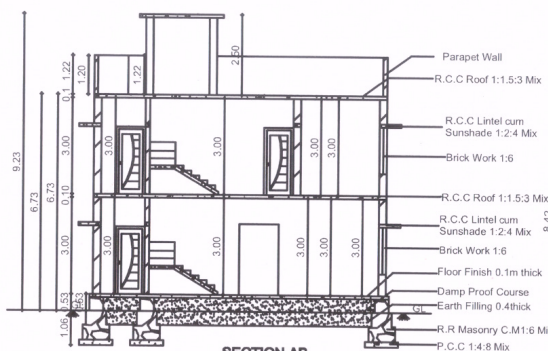
SECTION AB
