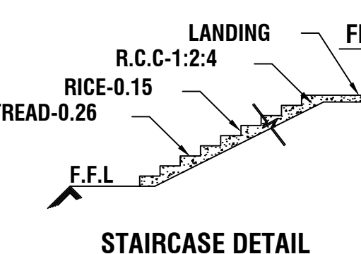
STAIRCASE DETAIL
