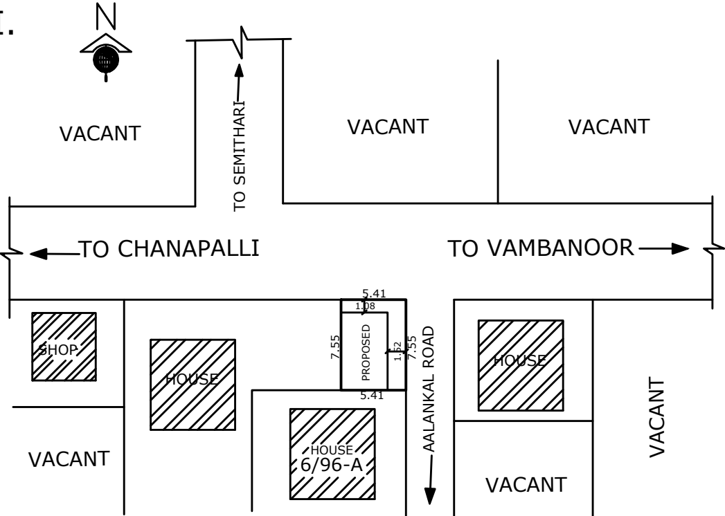
KEY PLAN [SCALE 1:400]
