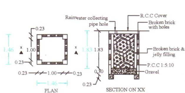
RAIN WATER HARVEST WELL RWH CAPACITY 1-6642LTRS
