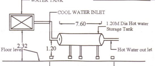
SOLAR WATER HEATING SYSTEM (S.W.H.S.DETAILS)
