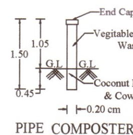
PIPE COMPOSTER
