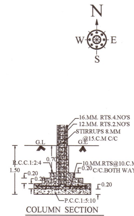
COLUMN SECTION
