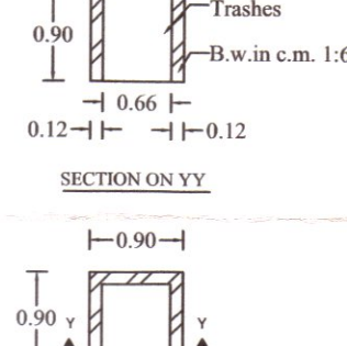
WASTE TRASH PIT
