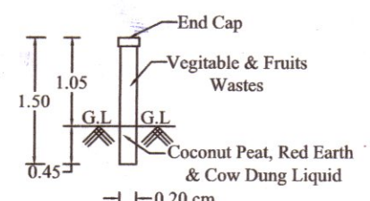
PIPE COMPOSTER
