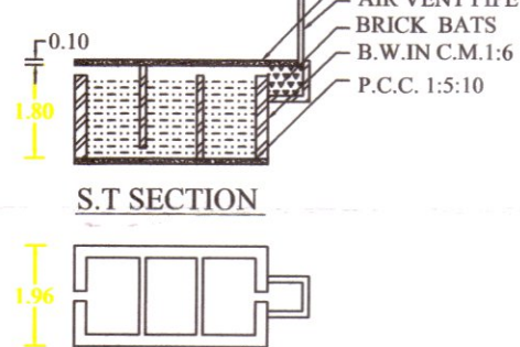
SEPTIC TANK PLAN
