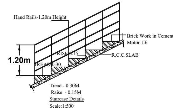
Hand Rail-1.20m Height
