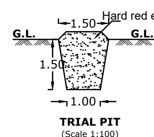
DETAILS OF RAIN WATER HARVESTING
