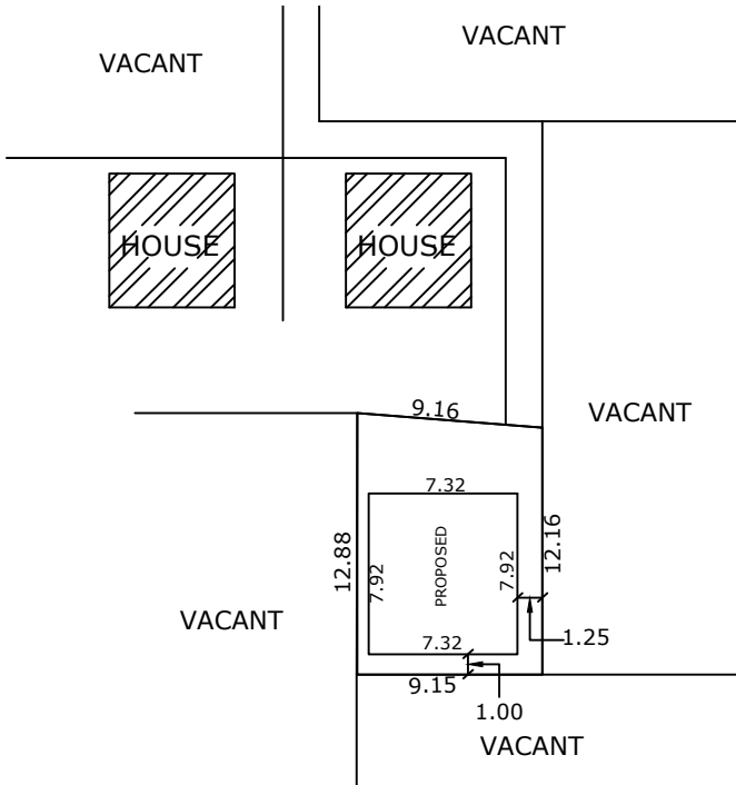
KEY PLAN [SCALE 1:400]
