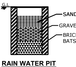
RAIN WATER PIT
