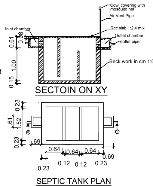
SEPTIC TANK PLAN
