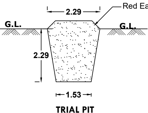
TRIAL PIT
