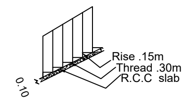
STAIRCASE DETAILS
