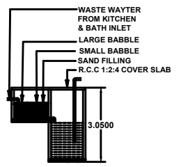
RECYCLING OF WASTE WATER TANK
