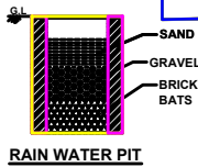
RAIN WATER PIT
