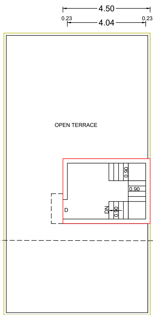
HEAD ROOM PLAN
