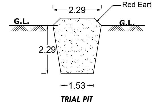
TRIAL PIT
