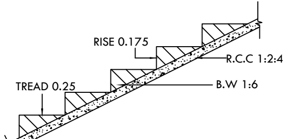
STAIR CASE DETAILS
