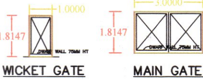
WICKET GATE
