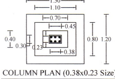
COLUMN PLAN (0.38x0.23 Size)
