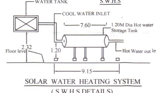
SOLAR WATER HEATING SYSTEM (S.W.H.S.DETAILS)
