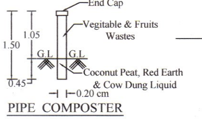
PIPE COMPOSTER
