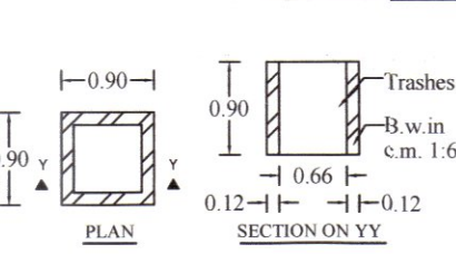
WASTE TRASH PIT
