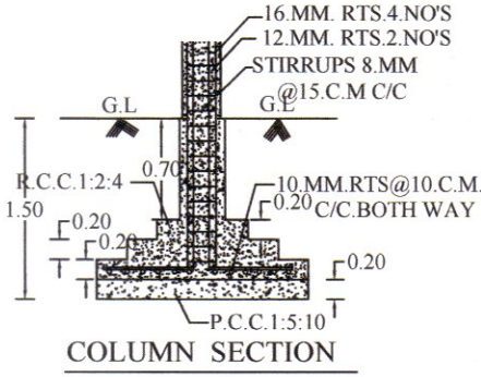
COLUMN SECTION
