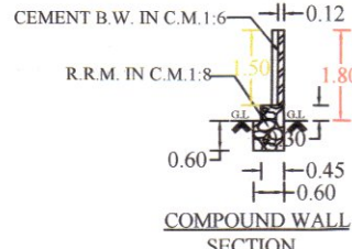
COMPOUND WALL SECTION
