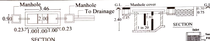
SECTION DETAILS OF SEPTIC TANK
