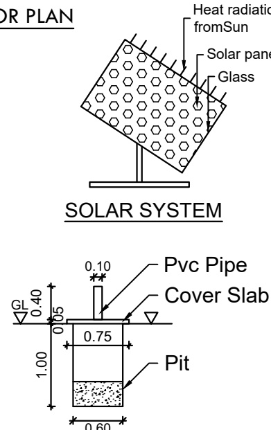
SOLAR SYSTEM
