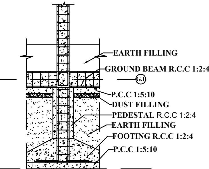
Details of R.C.C Column (Scale 1:100)
