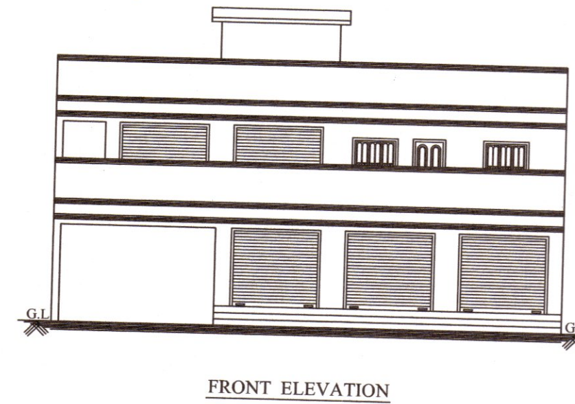
FRONT ELEVATION
