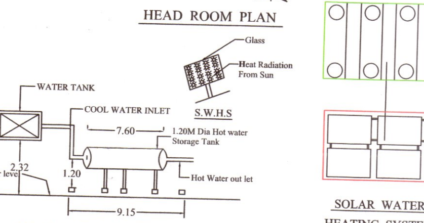
SOLAR WATER HEATING SYSTEM (S.W.H.S. DETAILS)
