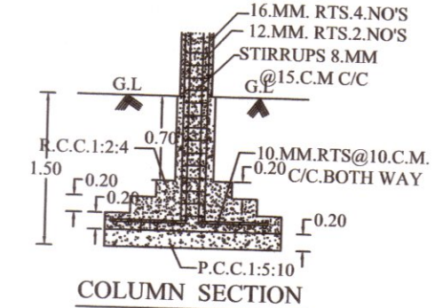
COLUMN SECTION
