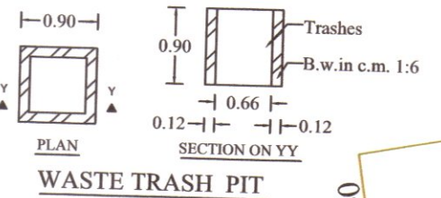
WASTE TRASH PIT
