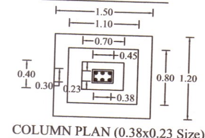
COLUMN PLAN (0.38x0.23 Size)
