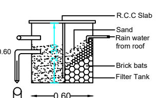
Details of Rain Water Harvesting
