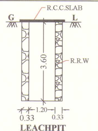
LEACH PIT
