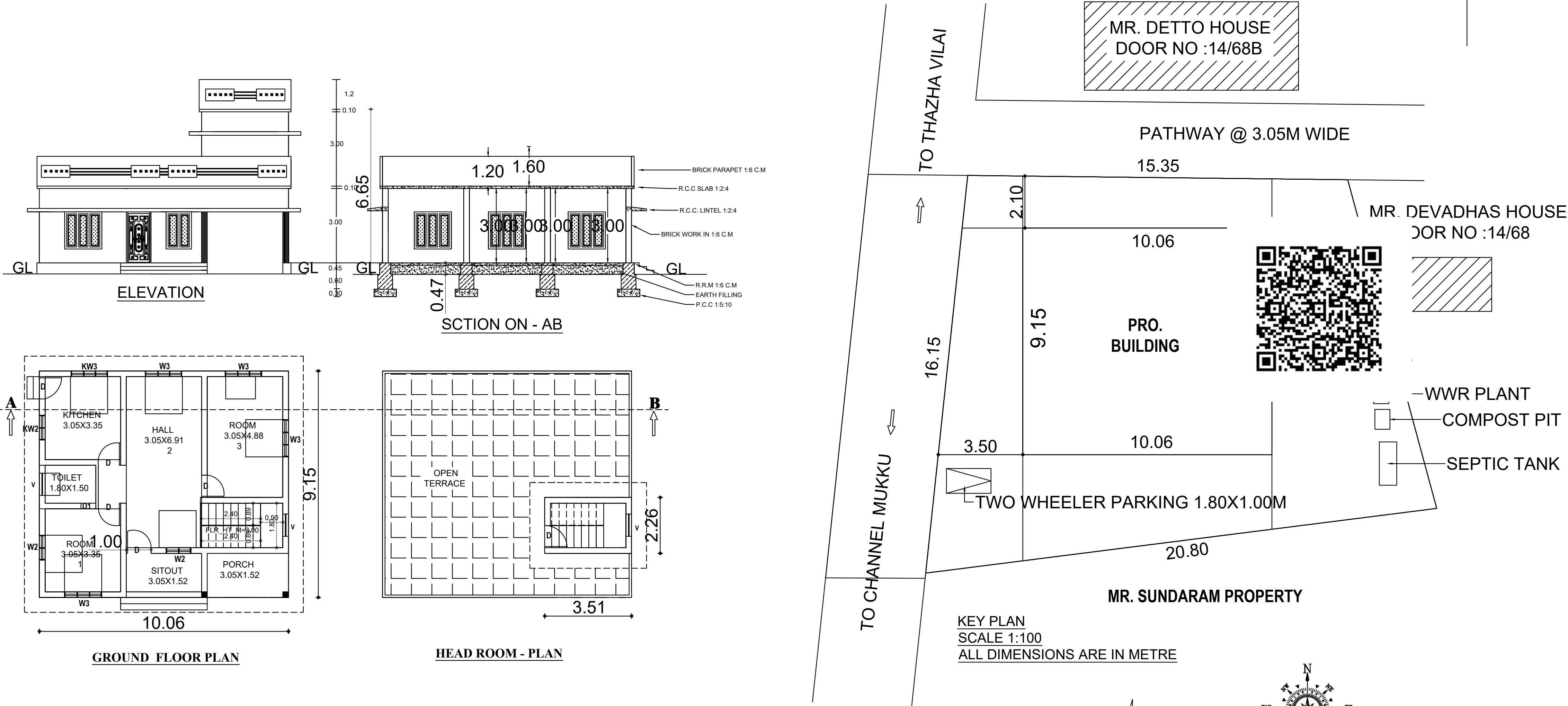
SCALE 1:100 ALL DIMENSIONS ARE IN METRE
