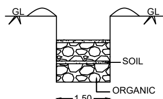
COMPOST PIT
