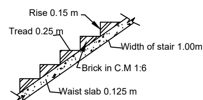
STAIR DETAILS
