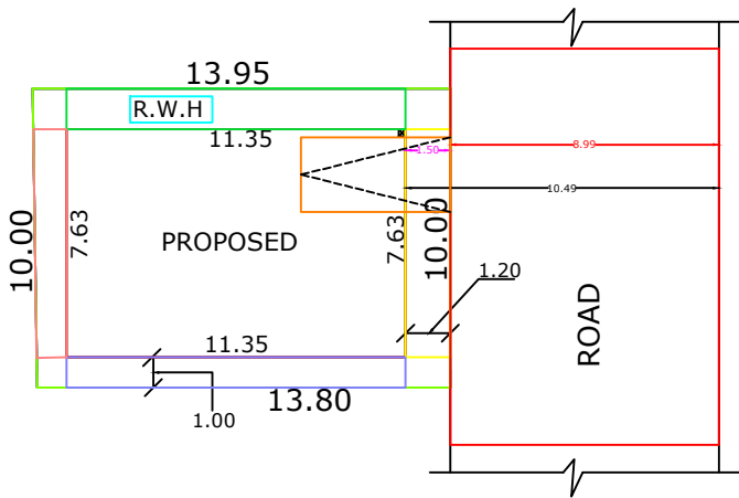
SITE PLAN [SCALE 1:100]
