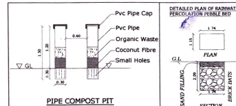
PIPE COMPOST PIT
