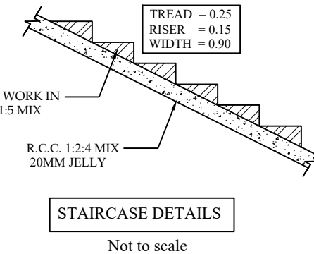
STAIRCASE DETAILS
