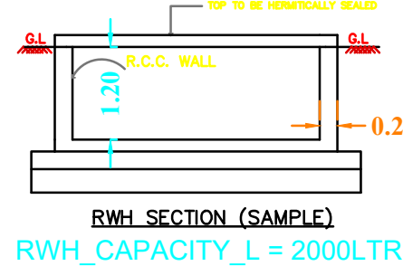
RWH SECTION (SAMPLE) RWH_CAPACITY_L = 2000LTRS
