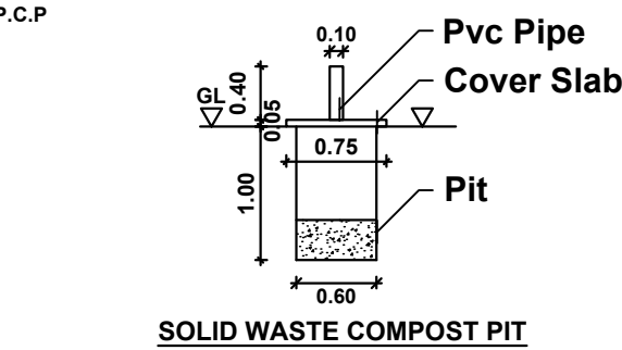
SOLID WASTE COMPOST PIT
