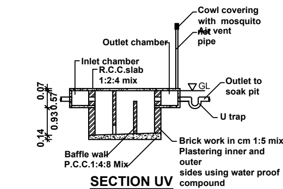
SECTION UV
