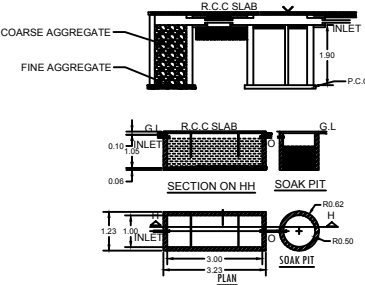
PLAN OF THE RAIN WATER COLLECTING TANK
