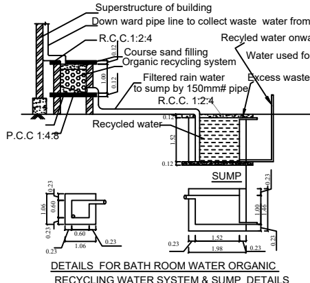
DETAILS FOR BATH ROOM WATER ORGANIC RECYCLING WATER SYSTEM & SUMP DETAILS
