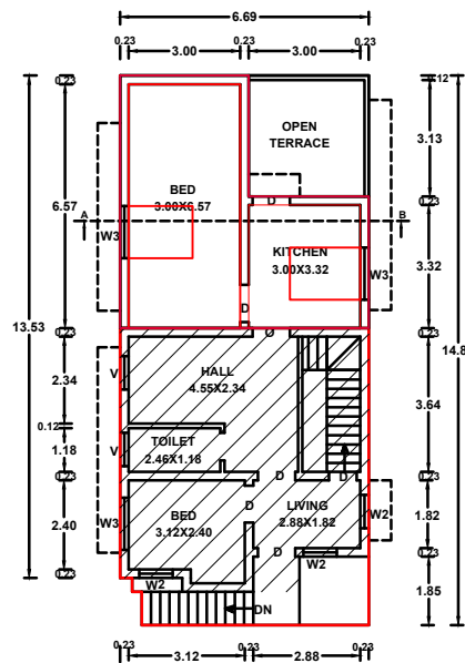
EXISTING, PROPOSED FIRST FLOOR PLAN
