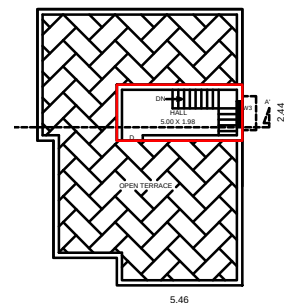
HEAD ROOM PLAN
