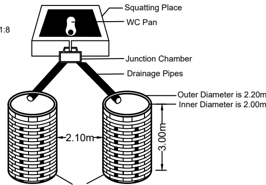
Twin Leach Pit
