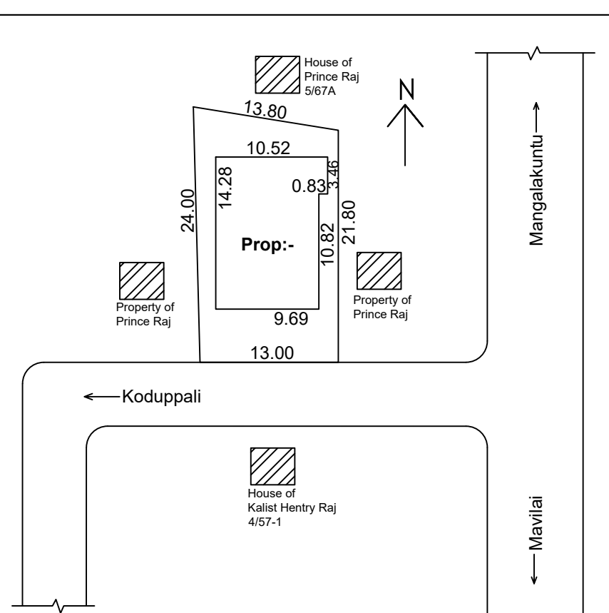
KEY PLAN SCALE 1:400
