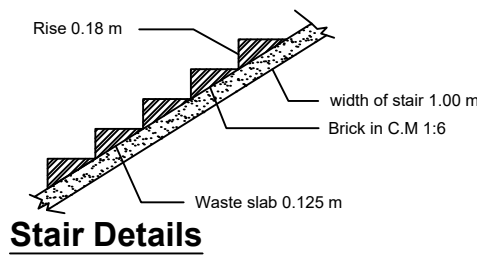
Stair Details
