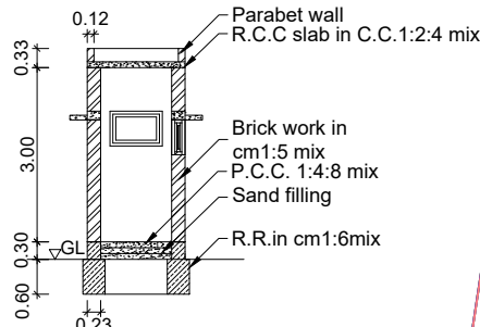
SECTION ON ST
