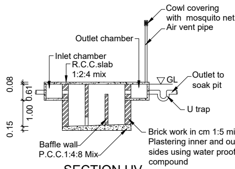
SECTION UV
