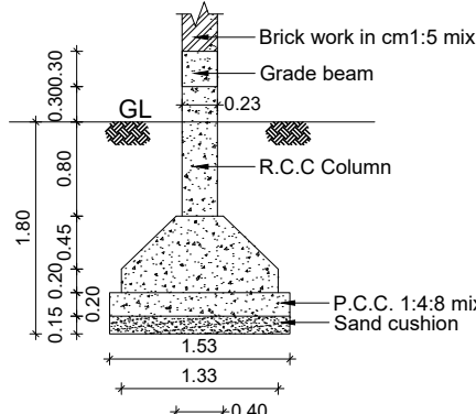
COLUMN DETAILS SCALE 1:50
