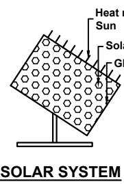
SOLAR SYSTEM
