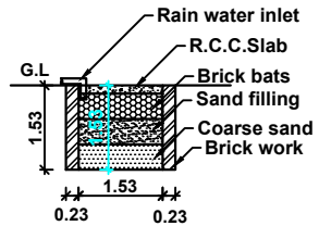
RAIN WATER HARVESTING PIT RWL_CAPACITY_L=5000LTRS
