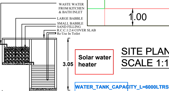
RECYCLING OF WASTE WATER FROM KITCHEN & BATHROOM
