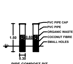
PIPE COMPOST PIT
