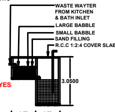
RECYCLING OF WASTE WATER TANK
