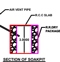
SECTION OF SOAKPIT
