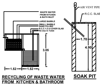
RECYCLING OF WASTE WATER FROM KITCHEN & BATHROOM
