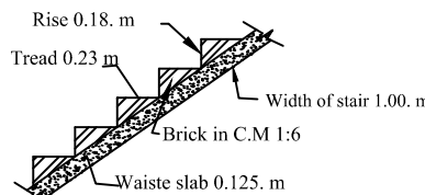
Stair Details
