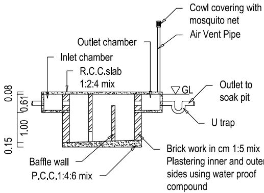
SECTION UV
