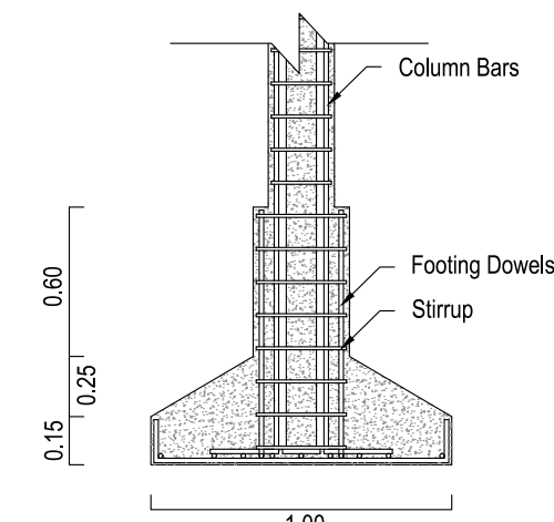
SECTION ON COLUMN FOUNDATION
