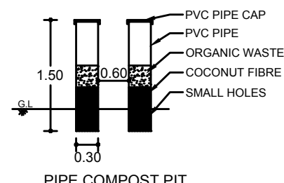
PIPE COMPOST PIT
