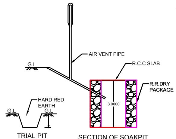
SECTION OF SOAKPIT
