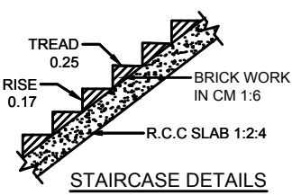
STAIRCASE DETAILS
