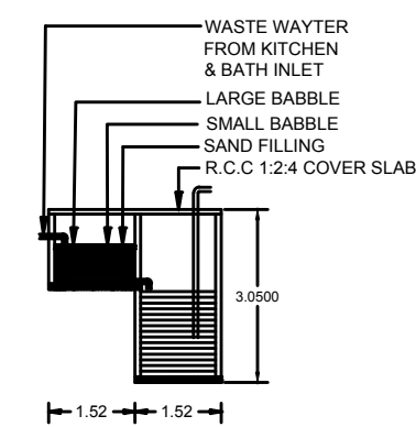
RECYCLING OF WASTE WATER TANK
