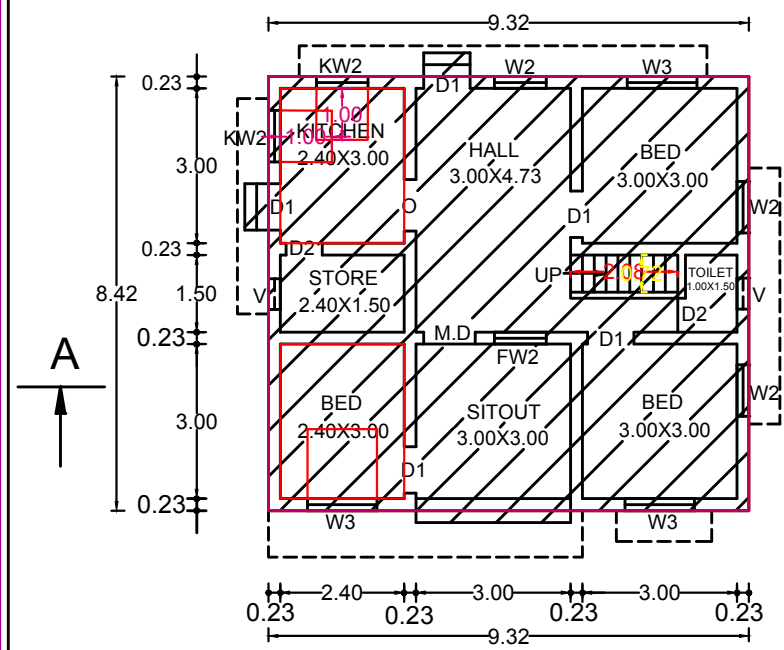
EXG.GROUND FLOOR PLAN
