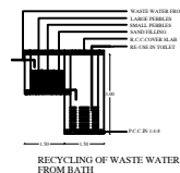
RECYCLING OF WASTE WATER FROM BATH
