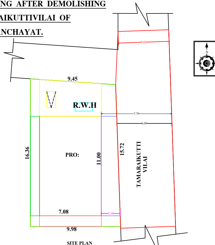
SITE PLAN
