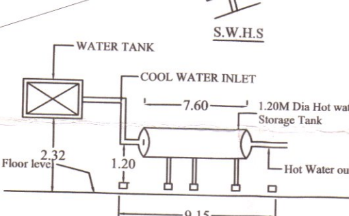
SOLAR WATER HEATING SYSTEM (S.W.H.S.DETAILS)
