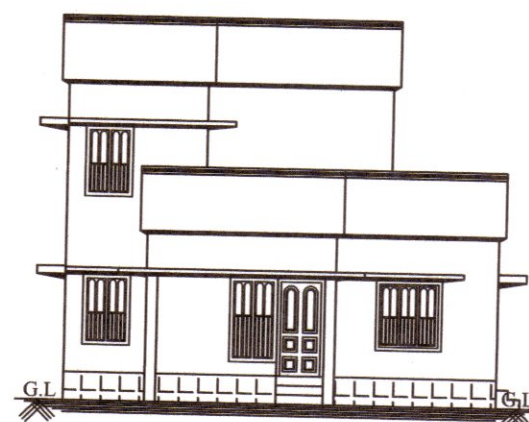
FRONT ELEVATION
