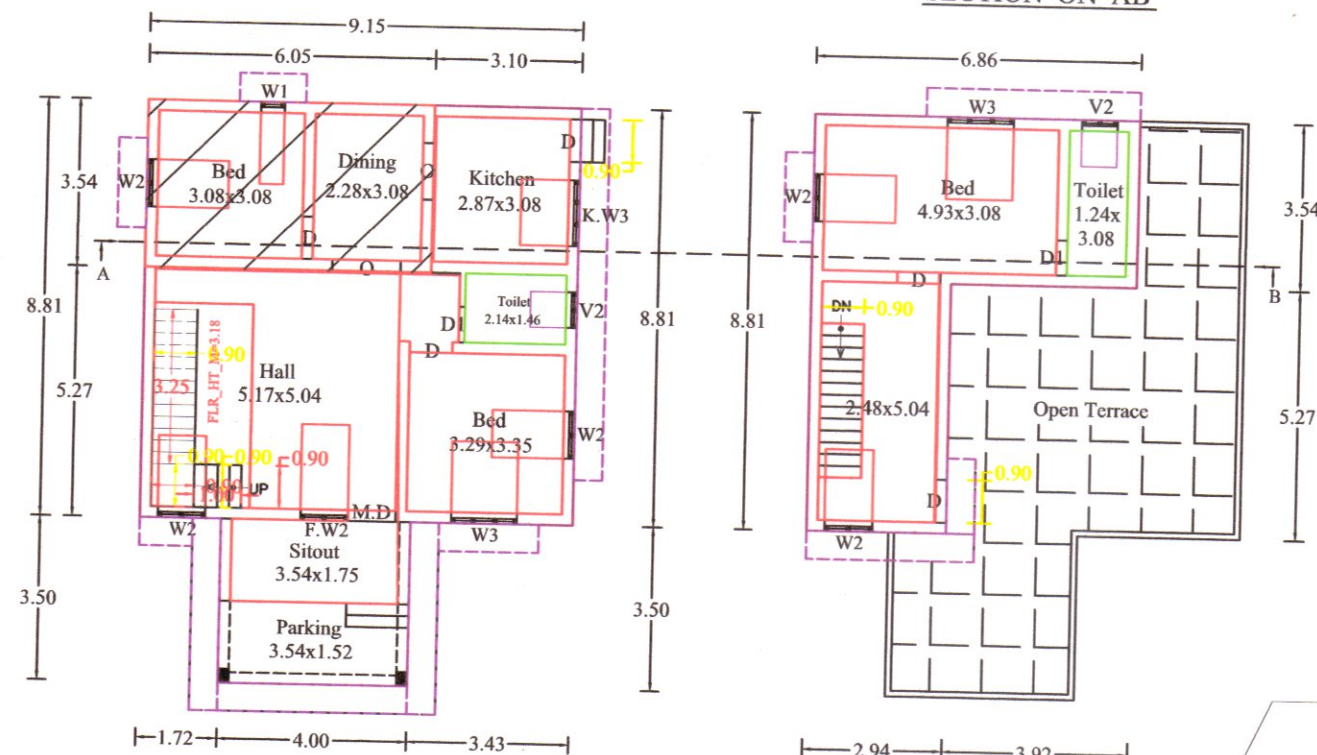
EXISTING & EXTENSION GROUND FLOOR PLAN DOOR NO :- 5/104/6
