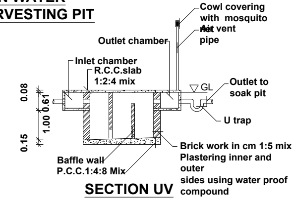
SECTION UV
