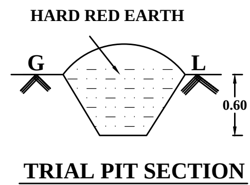
TRIAL PIT SECTION
