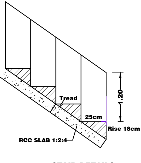
STAIR DETAILS
