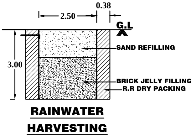
RAINWATER HARVESTING
