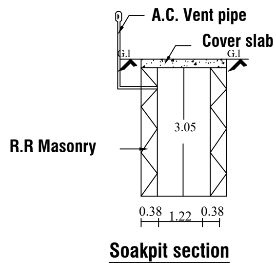
Soakpit section
